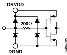
Figure 5. Three-State (OEB)
