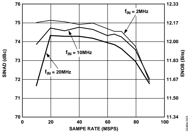
Figure 23. SINAD vs. Sample Rate
