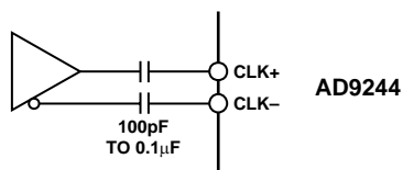
Figure 58. Differential Clock Input, AC-Coupled
