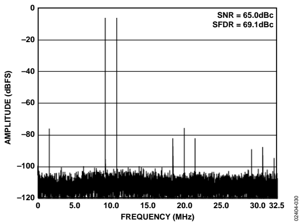
Figure 30. Dual-Tone FFT with f_{IN-1} = 139.2 MHz and f_{IN-2} = 140.7 MHz ( A_{IN1} = A_{IN2} = -6.5 dBFS)
