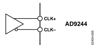
Figure 55. Differential Clock Input, DC-Coupled
