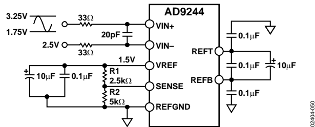
Figure 50. Resistor Programmable Reference (1.5 V p-p Input Span, Differential Input with VCM = 2.5 V)
