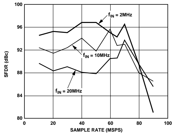
Figure 26. SFDR vs. Sample Rate
