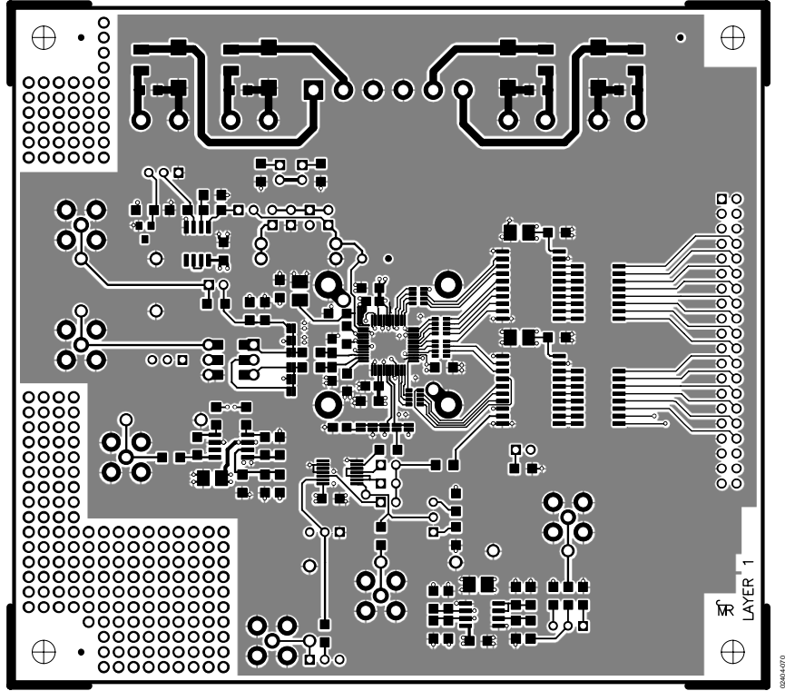
Figure 70. AD9244 Evaluation Board, PCB Layer 1 (Top)
