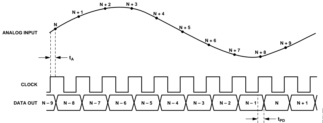
Figure 2. Input Timing
