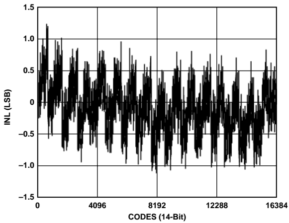
Figure 24. Typical INL
