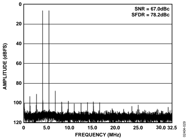
Figure 29. Dual-Tone FFT with f_{IN-1} = 69.2 MHz and f_{IN-2} = 70.6 MHz ( A_{IN1} = A_{IN2} = -6.5 dBFS)
