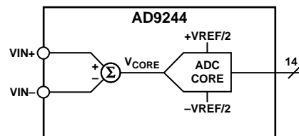
Figure 43. Equivalent Analog Input of AD9244
