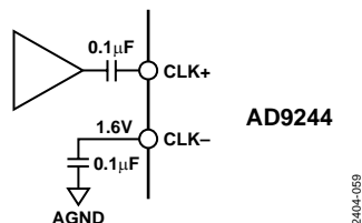
Figure 59. Single-Ended Clock Input, AC-Coupled
