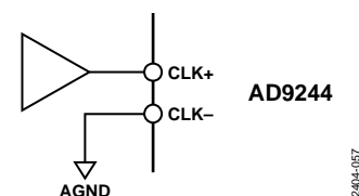
Figure 57. Single-Ended Input, Retains Pin Compatibility with AD9226
