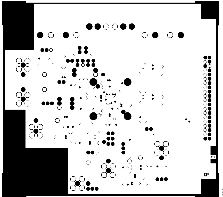
Figure 71. AD9244 Evaluation Board, PCB Layer 2 (Ground Plane)
