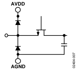
Figure 7. VIN+, VIN-
