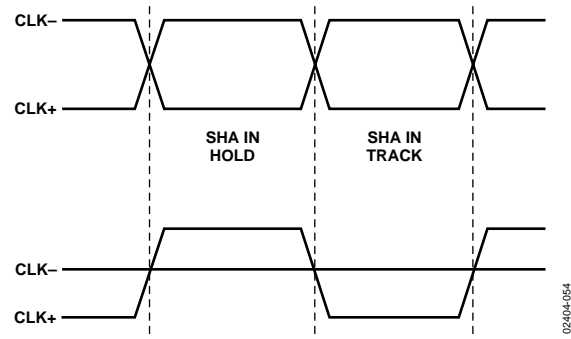
Figure 54. SHA Timing
