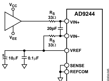
Figure 45. Resistors Isolating SHA Input from Op Amp
