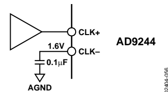
Figure 56. Single-Ended Clock Input, DC-Coupled
